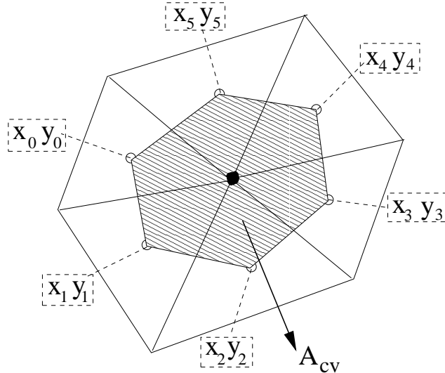
Figure 8.4: Control volume (centroid dual) of vertex is shaded. Some notation is introduced.
